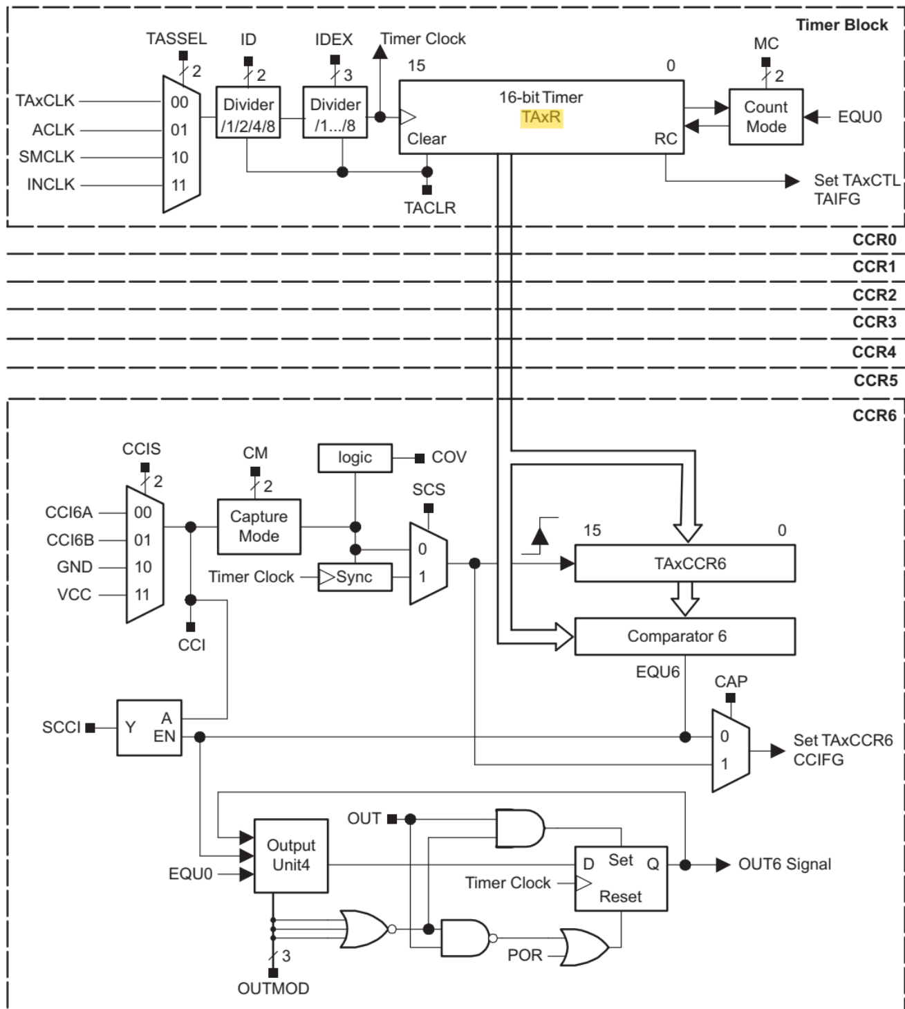
Figure 17-1. Timer_A Block Diagram
