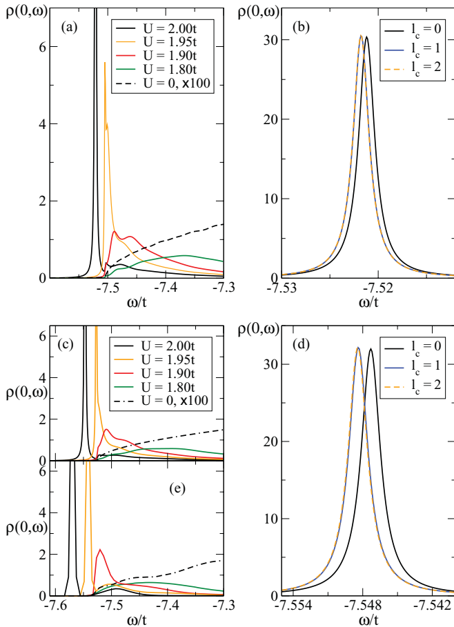
FIG. 3. (Color online) LDOS at the impurity site \rho(0,\omega) in units of 1/t vs the energy \omega/t for (a) MA (0) with l_c = 0 for U = 1.8, 1.9, 1.95 , and 2.0 . The dashed line shows the DOS for the clean system times 100, (b) MA (0) at U/t = 2 and cutoffs in the renormalized potential l_c = 0, 1, 2 . (c) and (d) are the same as (a) and (b), respectively, but using MA (1) . Panel (e) shows DMC results from Ref. 13, for same parameters as (a) and (b). Other parameters are \Omega = 2t , \lambda = 0.8 , and \eta/t = 10^{-3} .
