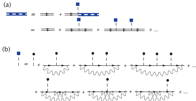
FIG. 2. (Color online) (a) Diagrammatic expansion for the full MA solution G_{ij}(\omega) (thick dashed blue line) in terms of the clean polaron Green's function (double thin line) and scattering on the renormalized disorder potential \epsilon_l^*(\omega) , depicted by dashed lines ended with squares. (b) Diagrammatic expansion of \epsilon_l^*(\omega) . For more details, see text.
