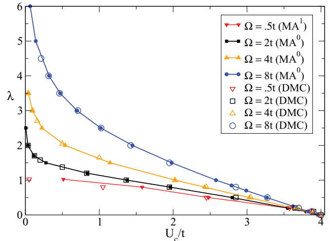
FIG. 4. (Color online) Phase diagram separating the regime where the polaron is mobile (below the line) and trapped (above the line). The effective coupling is \lambda = g^2/(6t\Omega) and the critical trapping potential U_c is shown for several values of \Omega/t . The MA results (filled symbols) compare well with the DMC results of Ref. 13 (empty symbols).
