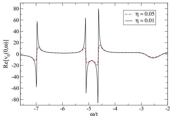
FIG. 6. (Color online) Real part of the additional on-site MA (0) disorder potential v_0(0, \omega) over a wide energy range for U = 2t , \Omega = 2t , \lambda = 0.8 , and two values of \eta .
