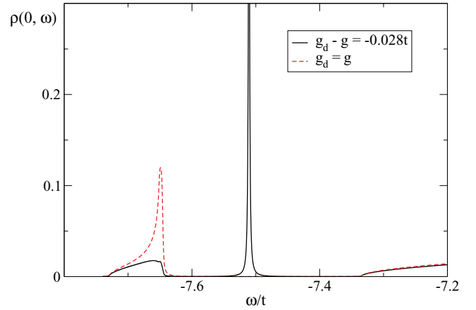
FIG. 8. (Color online) For large \lambda , in the clean system (dashed red line), the first polaron band is separated by an energy gap from the next features in the spectrum (here, the band associated with the second bound state). For g_d < g , an “antibound” impurity state is pushed inside this gap (black full line). Parameters are \Omega = t = 1 , \lambda = 1.2 , and \eta = 10^{-3} .
