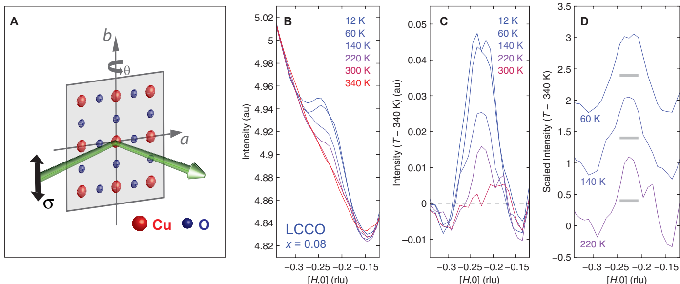
Fig. 1. CO in LCCO. (A) Scattering geometry along the Cu–O bond direction (see text for details). (B) RXS \theta scans for LCCO ( x = 0.08 , T_c \sim 20 K) at various temperatures. au, arbitrary units. (C) CO peaks at different temperatures obtained upon subtracting the 340 K data from those at lower temperatures. (D) Data (60, 140, and 220 K) from (C) with their maxima normalized to unit. The curves were offset for clarity, and the width of gray bars represents the half width at half maximum of the 60 K data.
